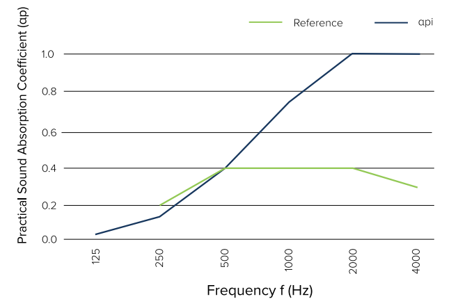
Sound absorption coefficient with reference curve
