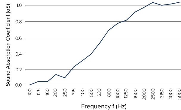
Sound absorption coefficient
